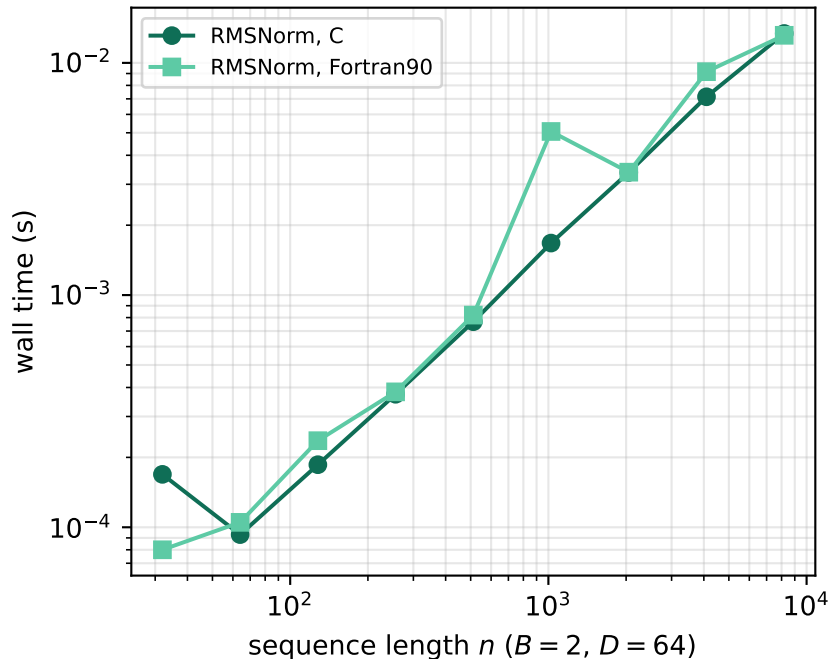
RMSNorm forward+backward
