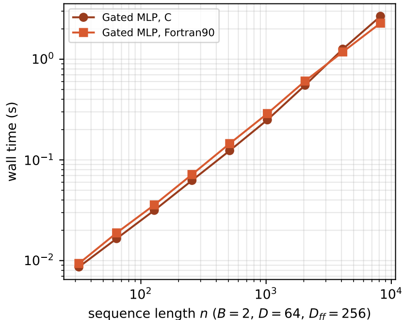
Gated MLP forward+backward
