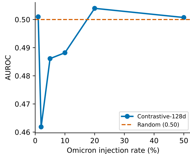
Anomaly AUROC vs Injection Rate
