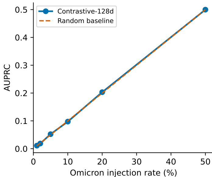
Anomaly AUPRC vs Injection Rate
