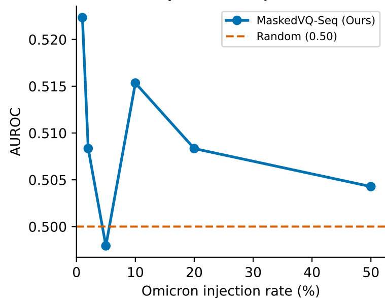
Anomaly AUROC vs Injection Rate
