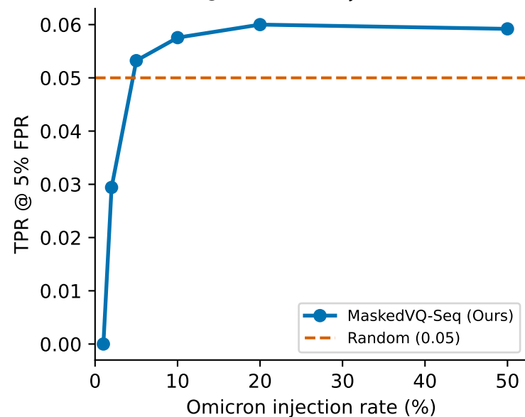
TPR @ 5% FPR vs Injection Rate
