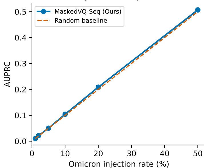
Anomaly AUPRC vs Injection Rate
