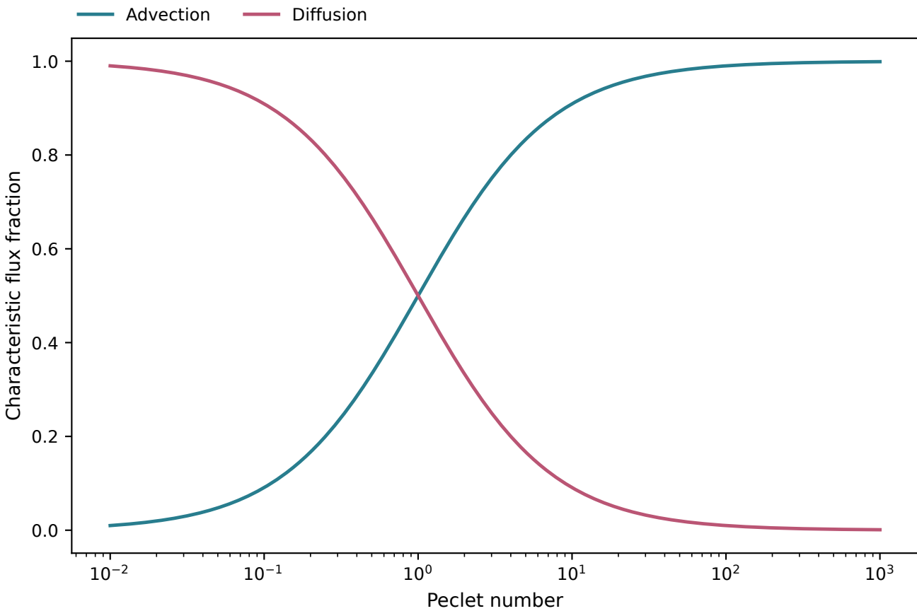
Peclet number and transport balance
