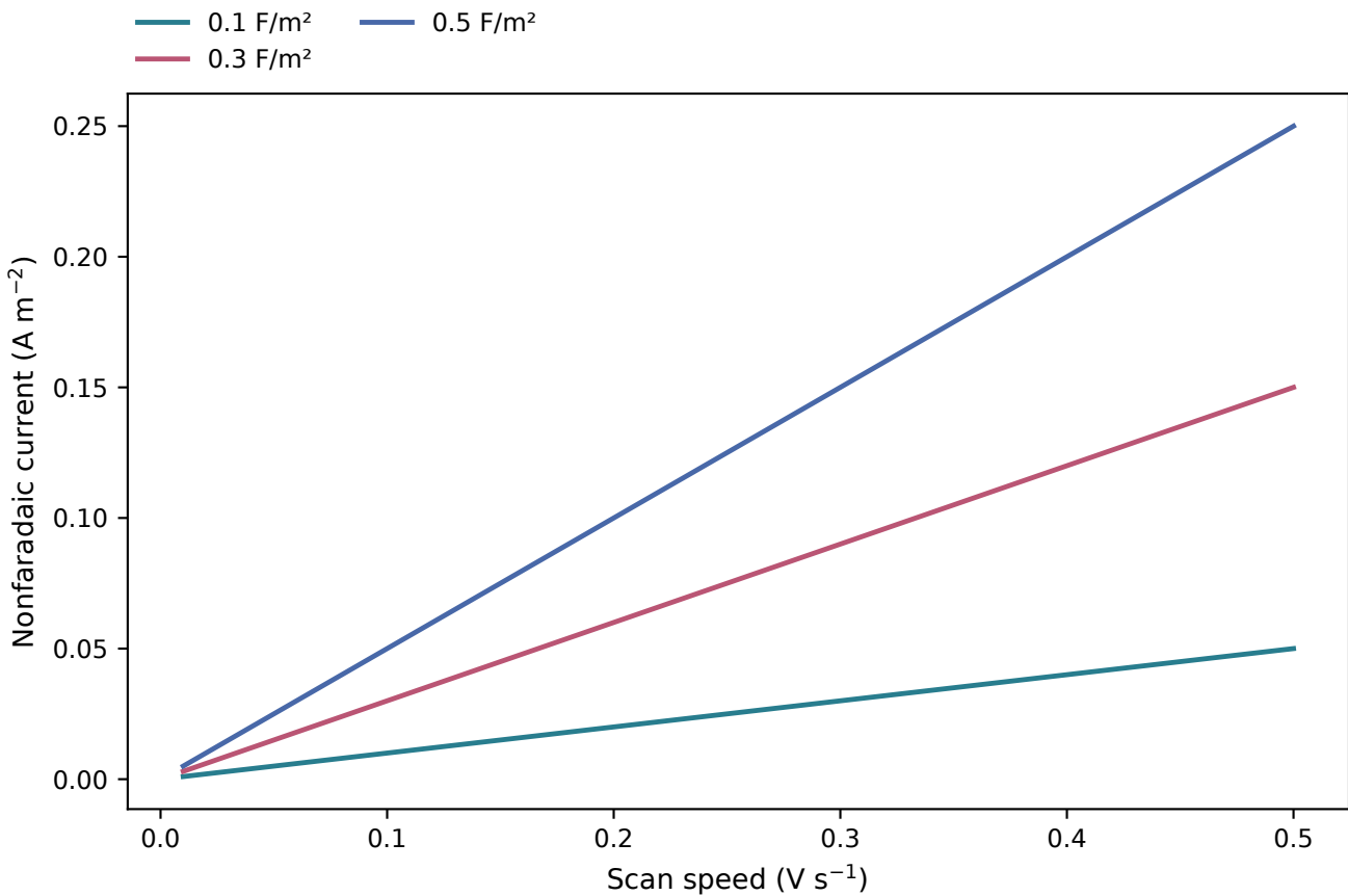
Scan speed and double-layer current
