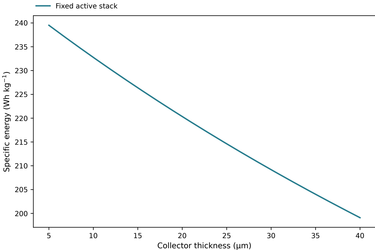
Collector thickness and specific energy
