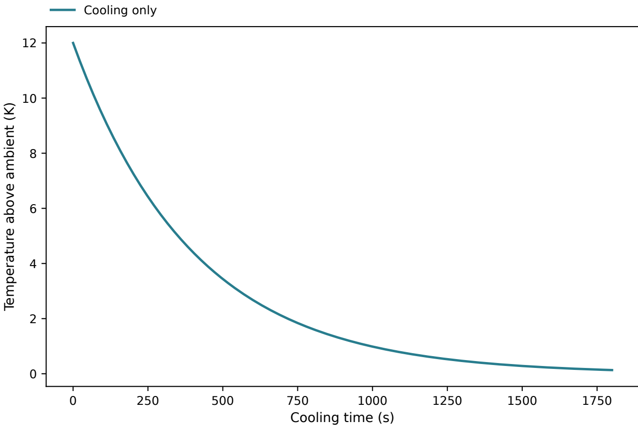
Temperature decay after heating stops
