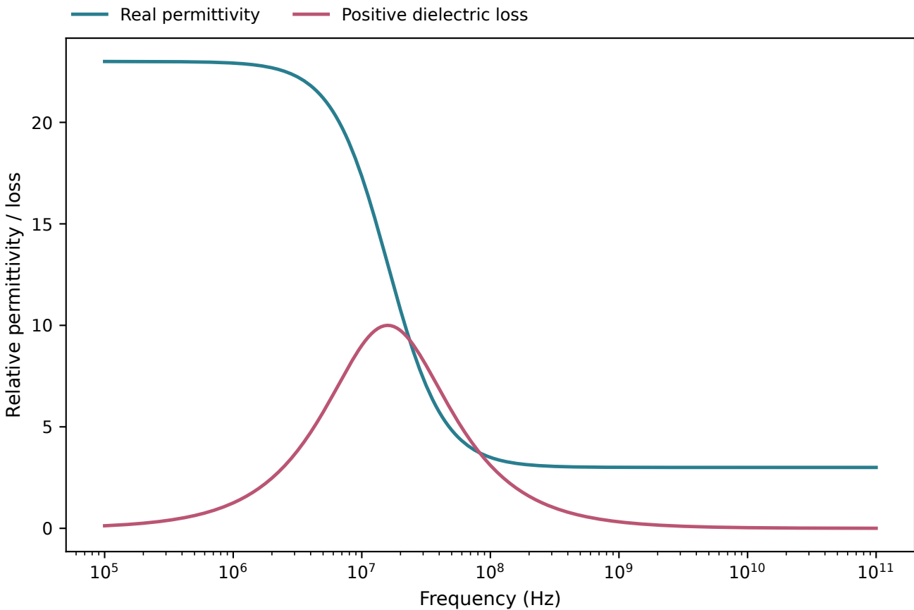
Frequency and dielectric relaxation loss
