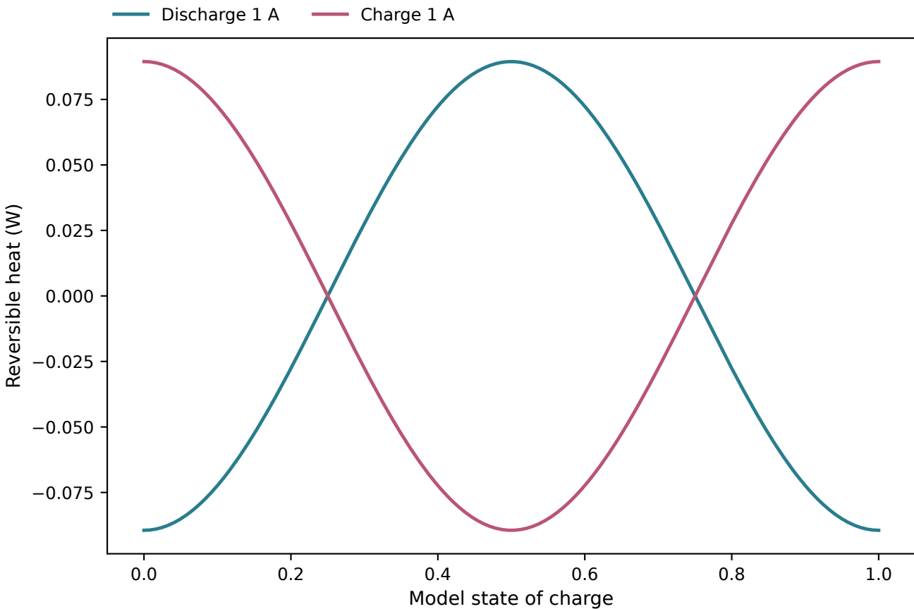
State of charge and reversible heat sign
