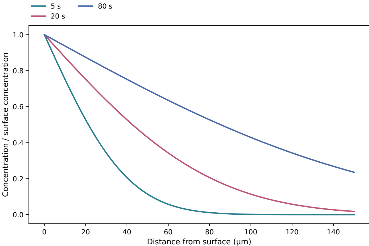
Diffusion time and penetration profile
