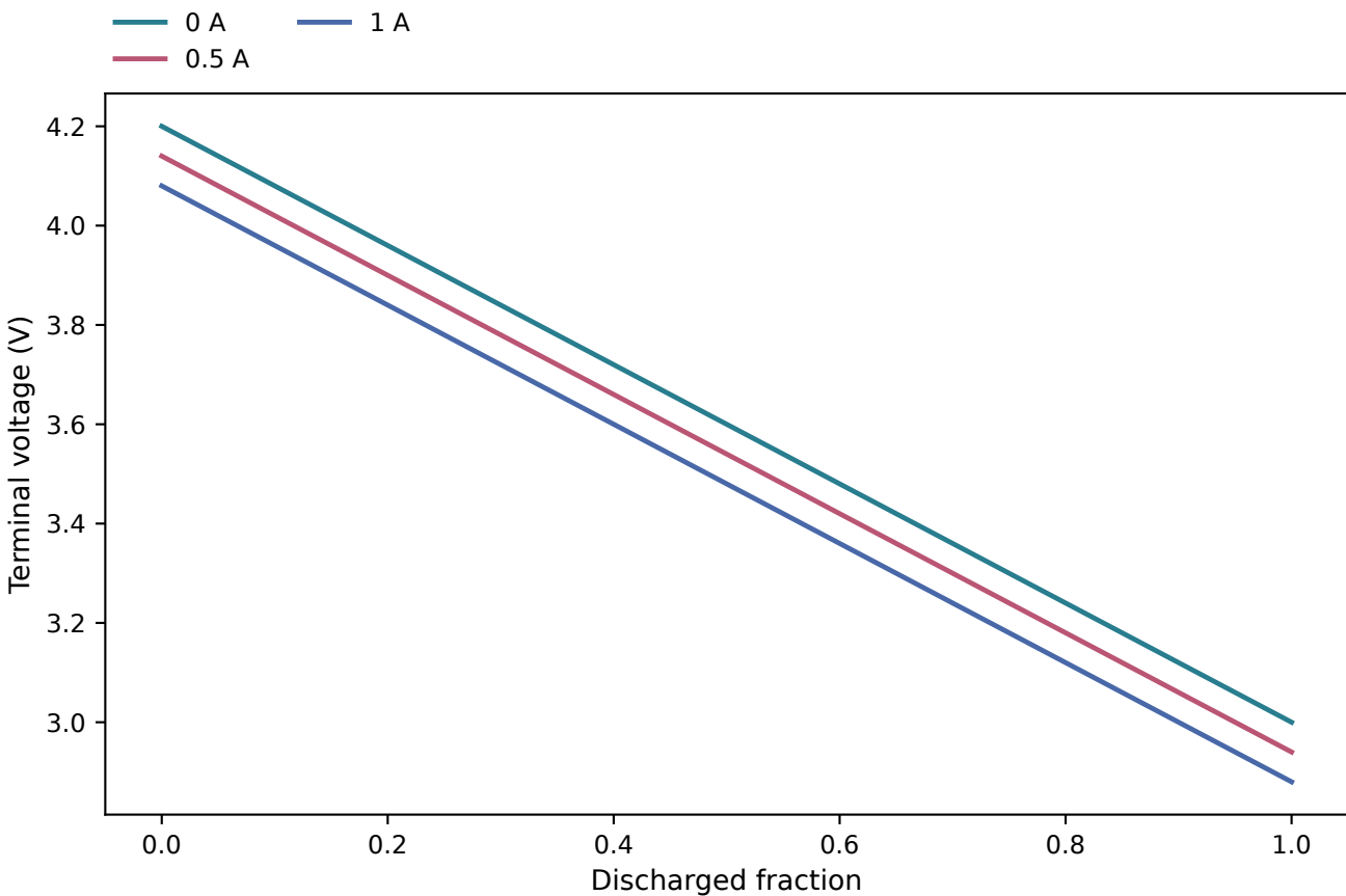
Ohmic drop and voltage cutoff
