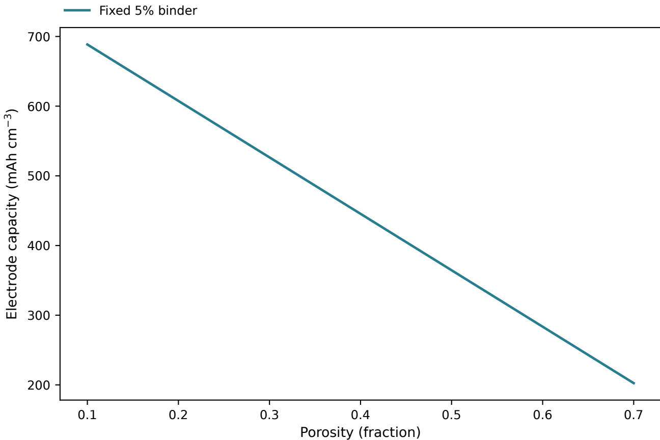
Porosity and volumetric capacity
