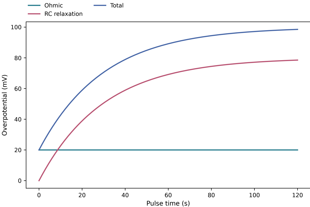
Pulse voltage contributions
