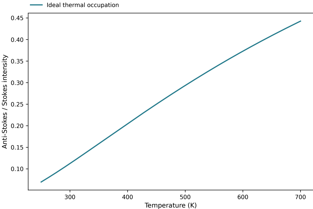
Temperature and anti-Stokes/Stokes ratio
