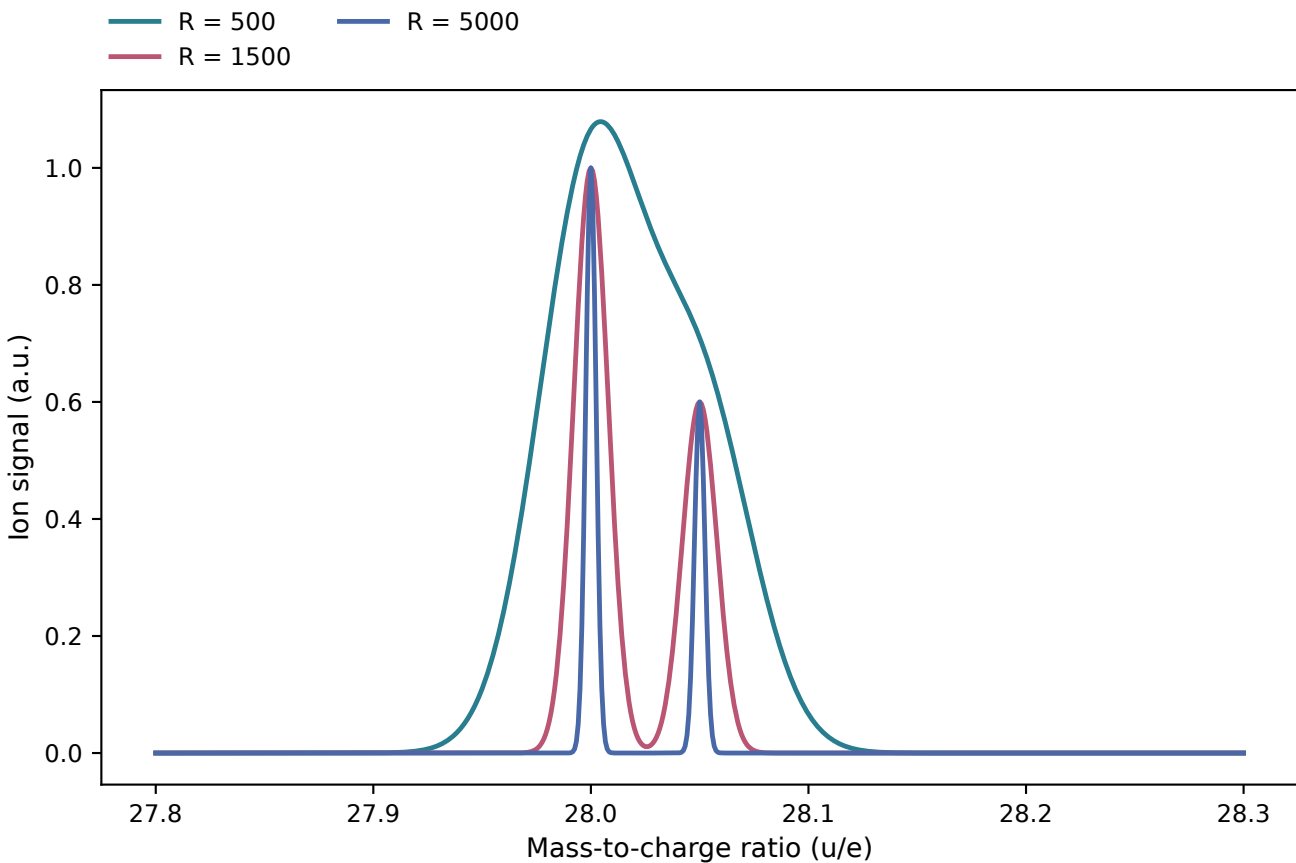
Mass resolution and ion-peak overlap
