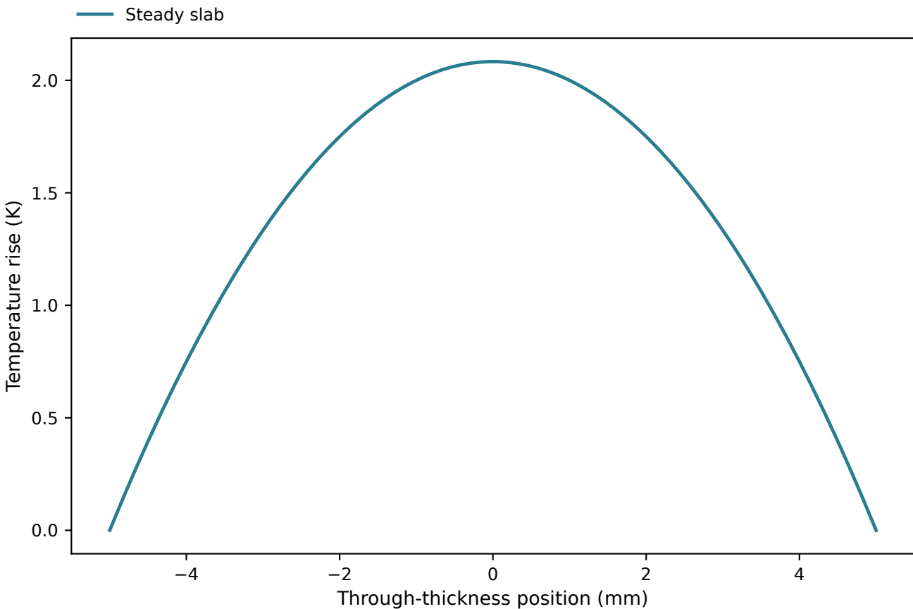
Slab temperature with internal heating
