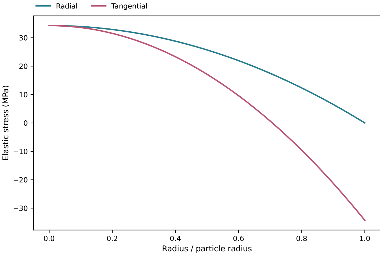
Spherical concentration gradient and stress
