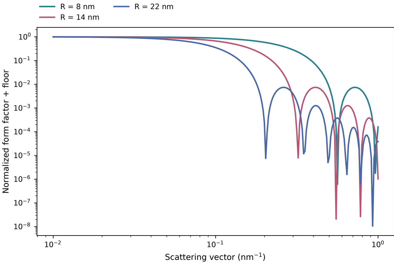
Sphere radius and form-factor minima
