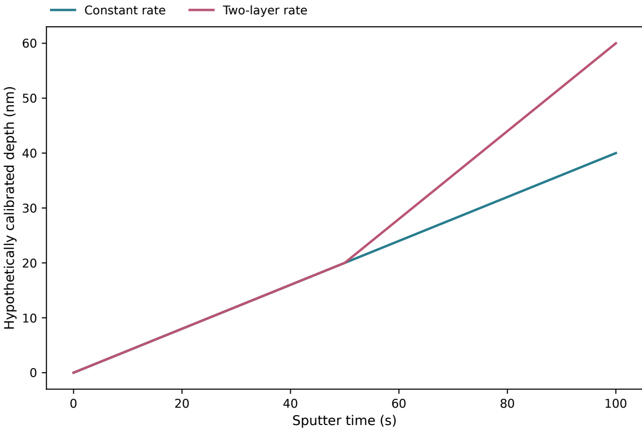
Variable sputter rate and depth calibration
