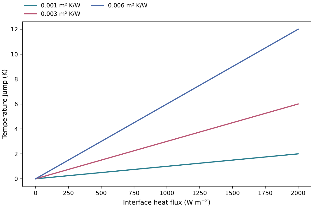
Interface heat flux and temperature jump
