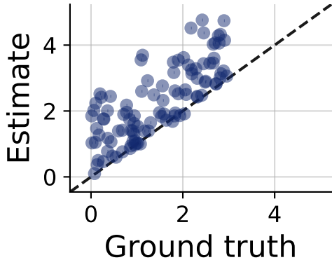
OLS
