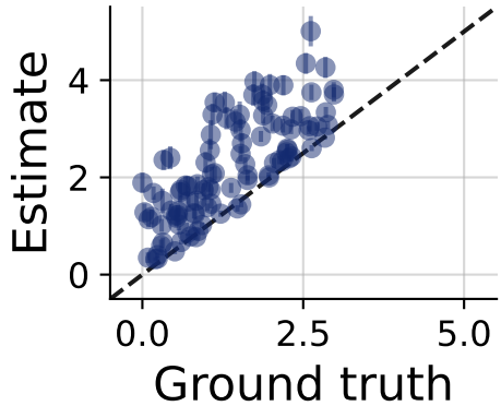
OLS
