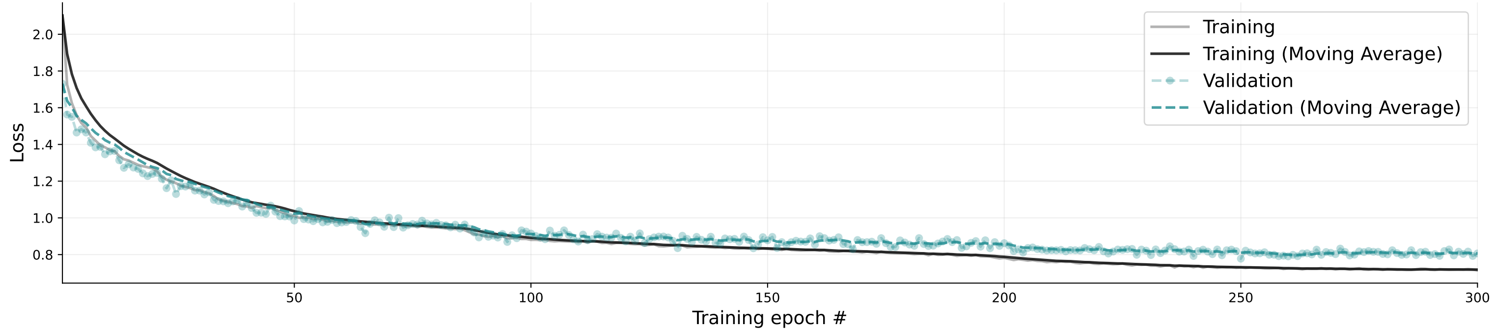
Loss Trajectory
