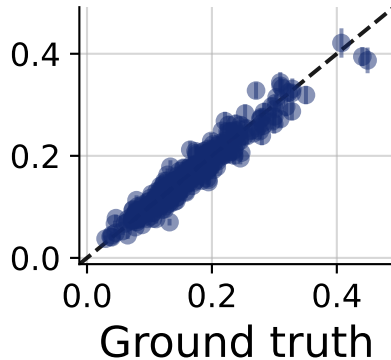
NPE Prevalence Prediction
