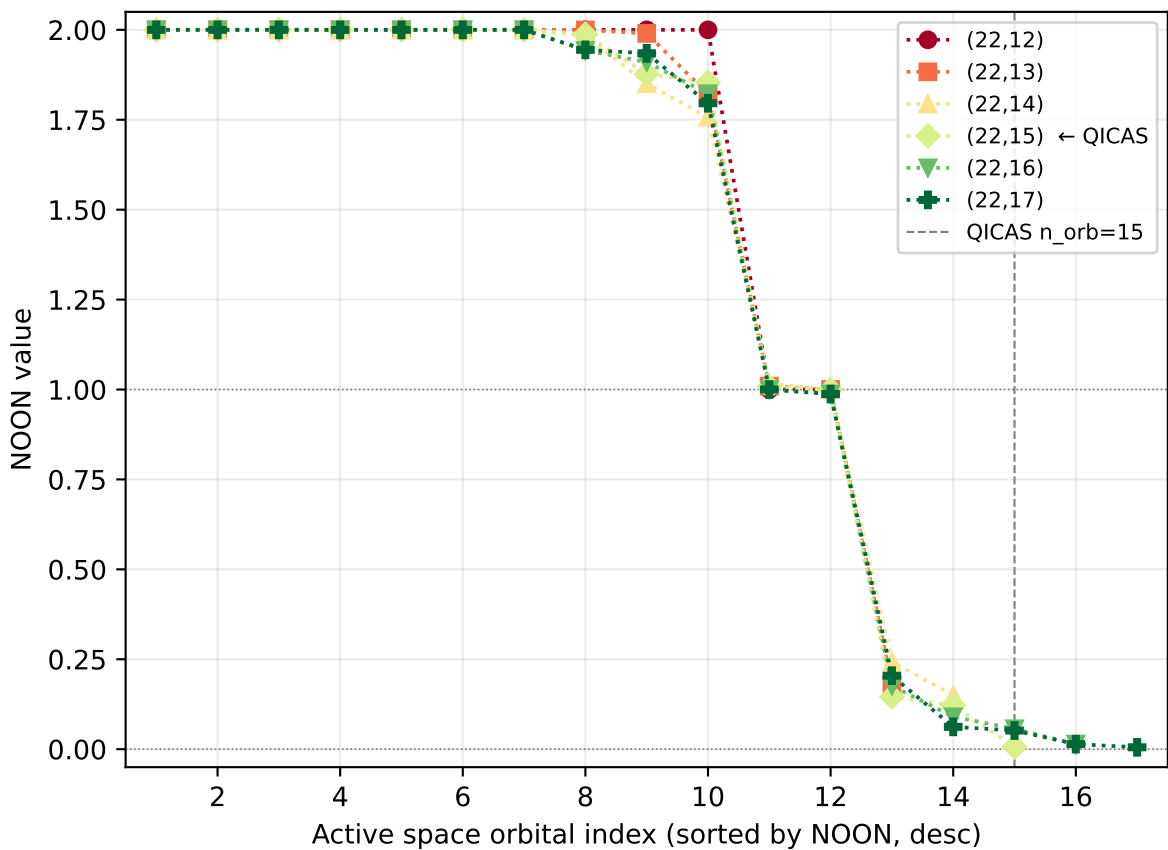
NOON convergence — VBr6_chg-3_spin2_oct
