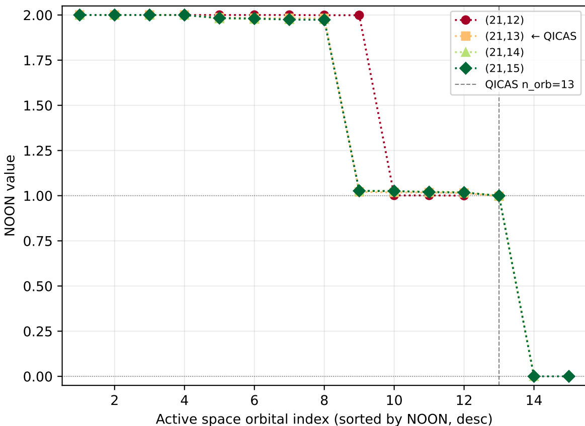
NOON convergence — MnCl 4 _chg-2_spin3_tet
