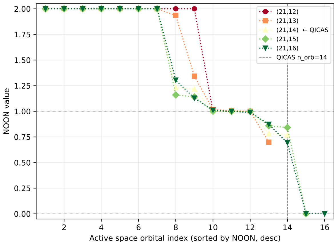
NOON convergence — V_Cl6_chg-2_spin3_oct_d2p394
