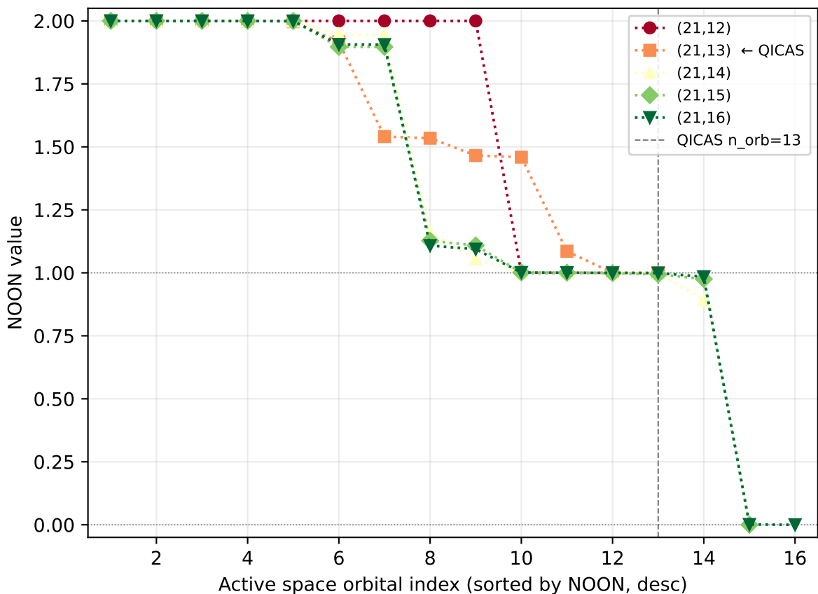
NOON convergence — MnBr4_chg-2_spin3_tet
