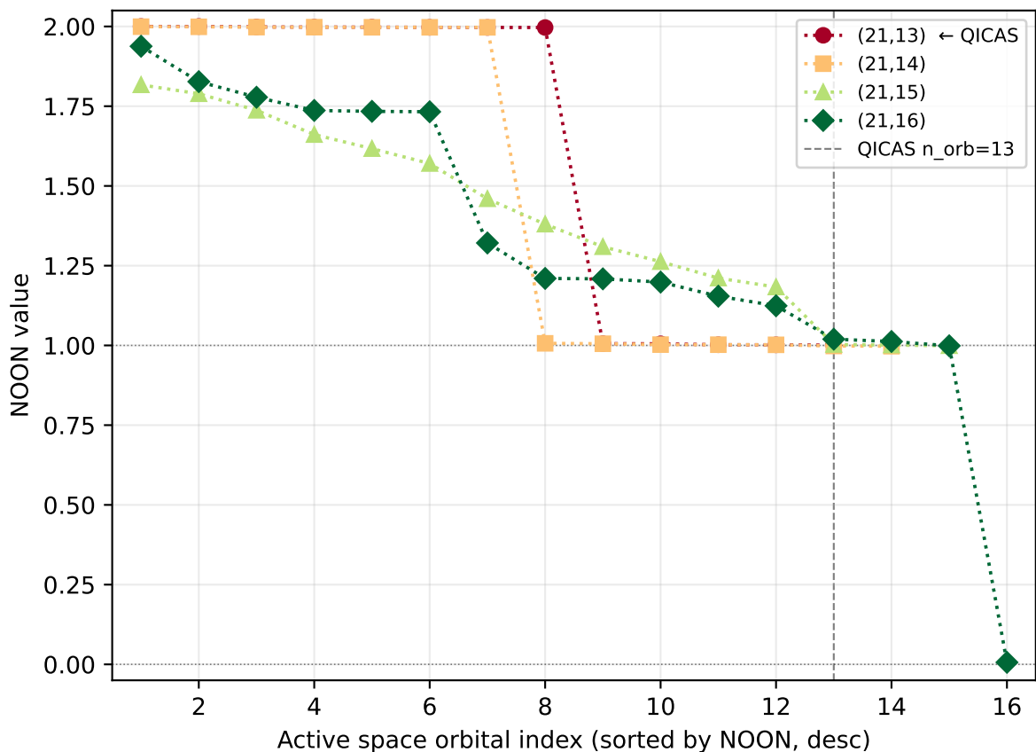
NOON convergence — MnBr4_chg-2_spin5_tet
