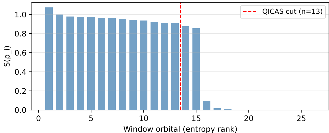
QICAS single-orbital entropy profile
