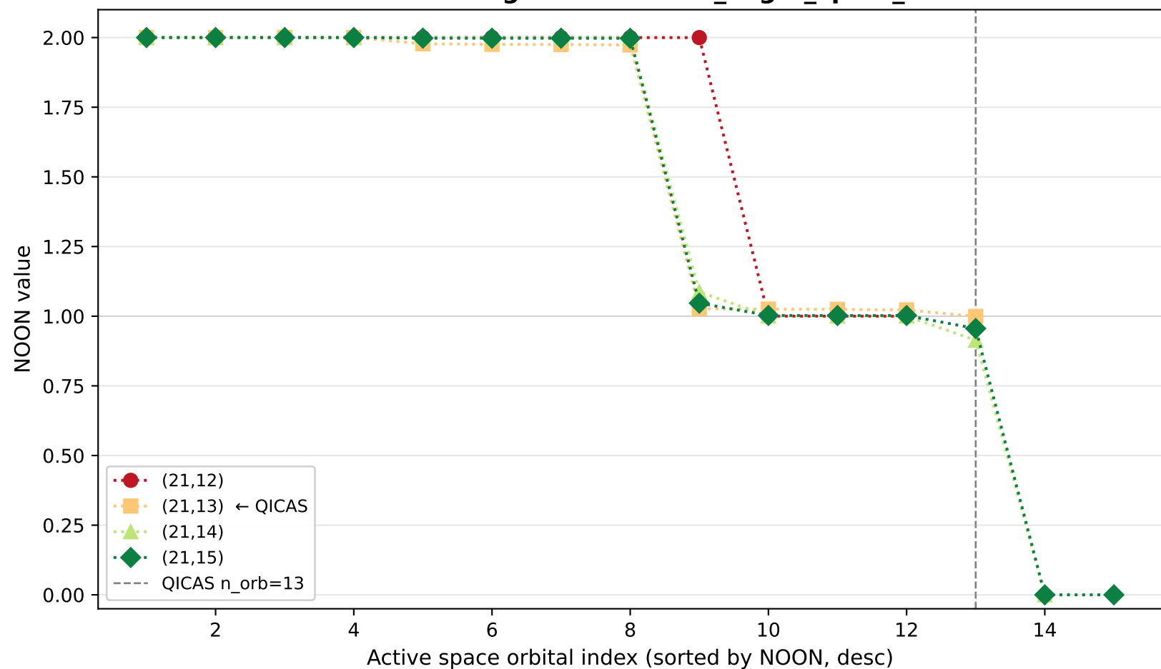
NOON convergence — MnCl4_chg-2_spin3_tet
