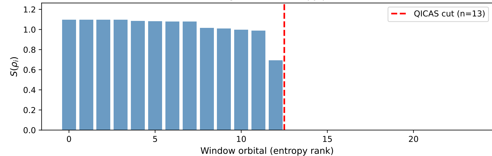
QICAS single-orbital entropy profile
