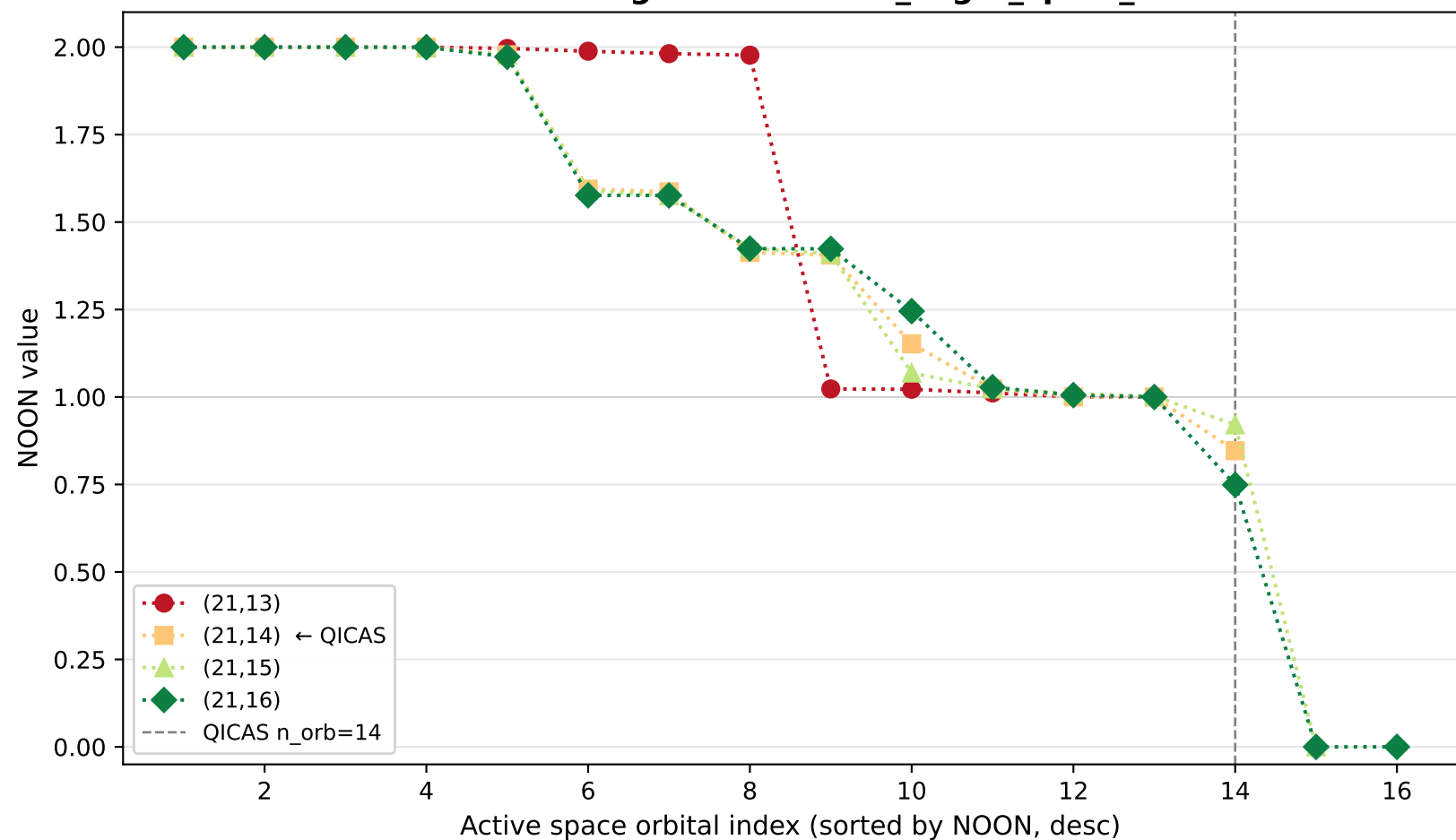
NOON convergence — MnCl4_chg-2_spin5_tet
