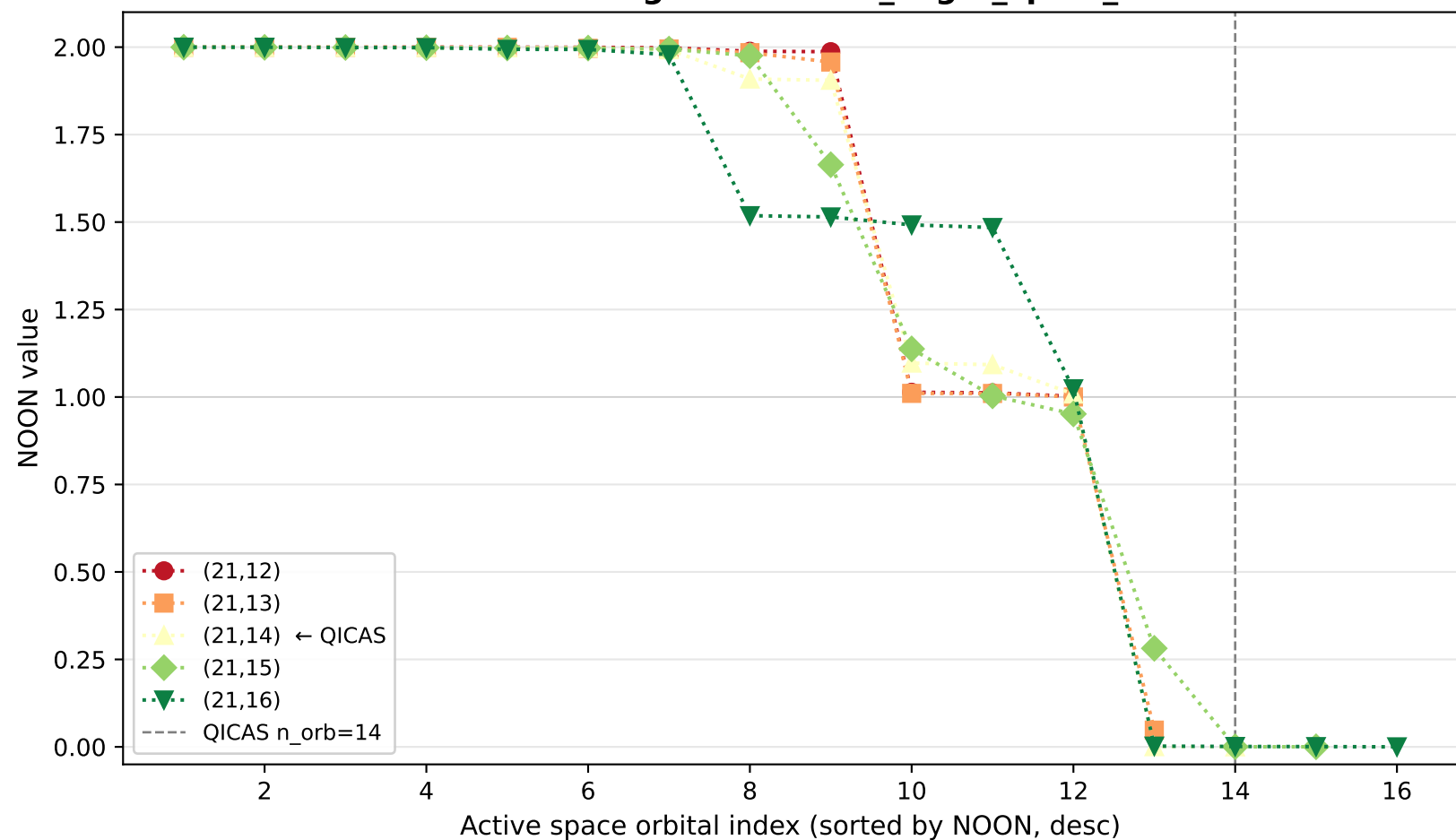
NOON convergence — VCI6_chg-2_spin3_oct
