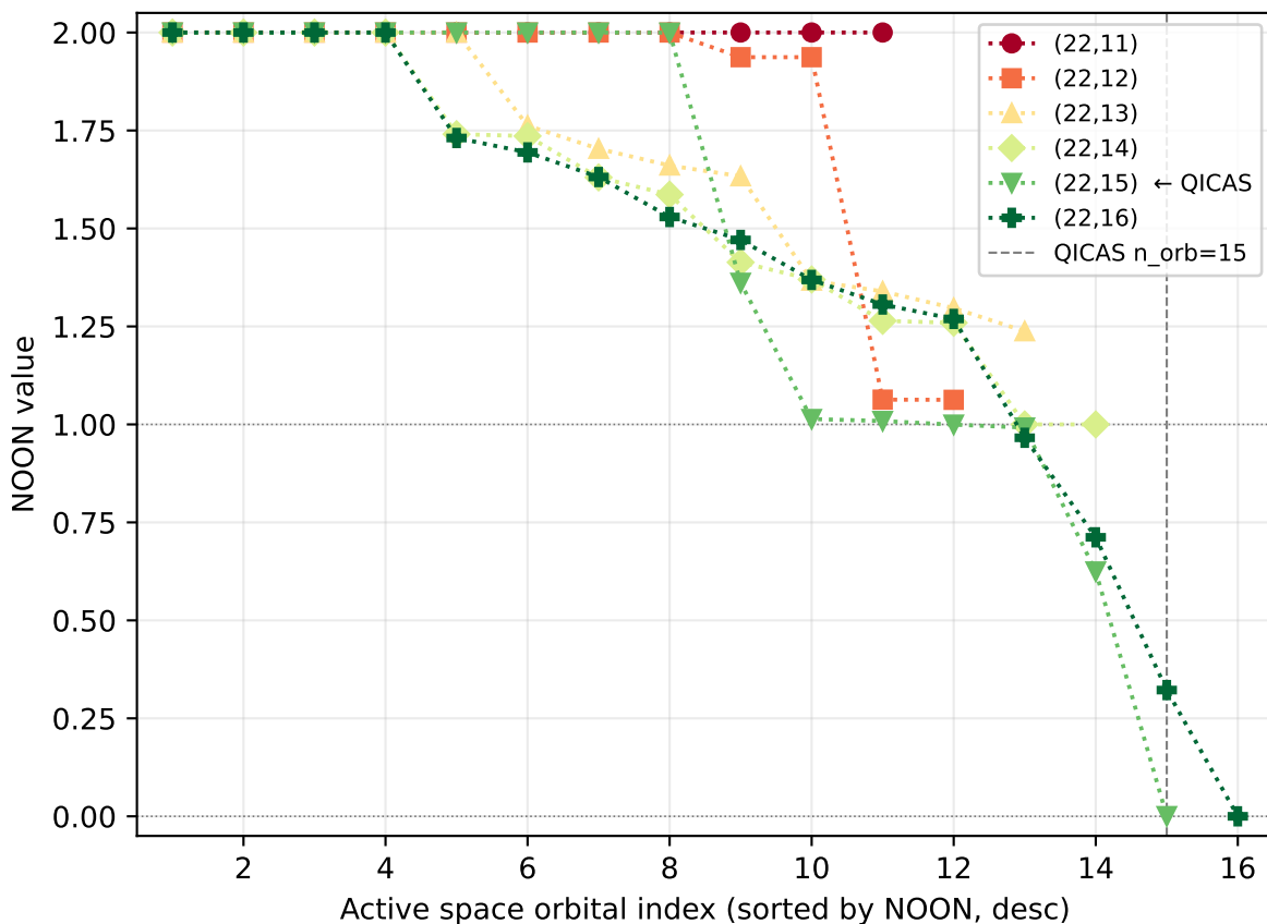
NOON convergence — MnBr4_chg-1_spin0_tet
