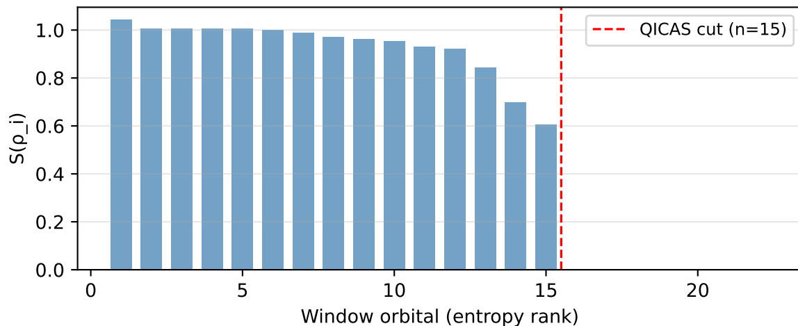
QICAS single-orbital entropy profile
