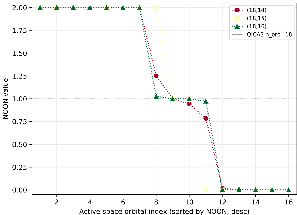
NOON convergence — NiBr6_chg-4_spin2_oct
