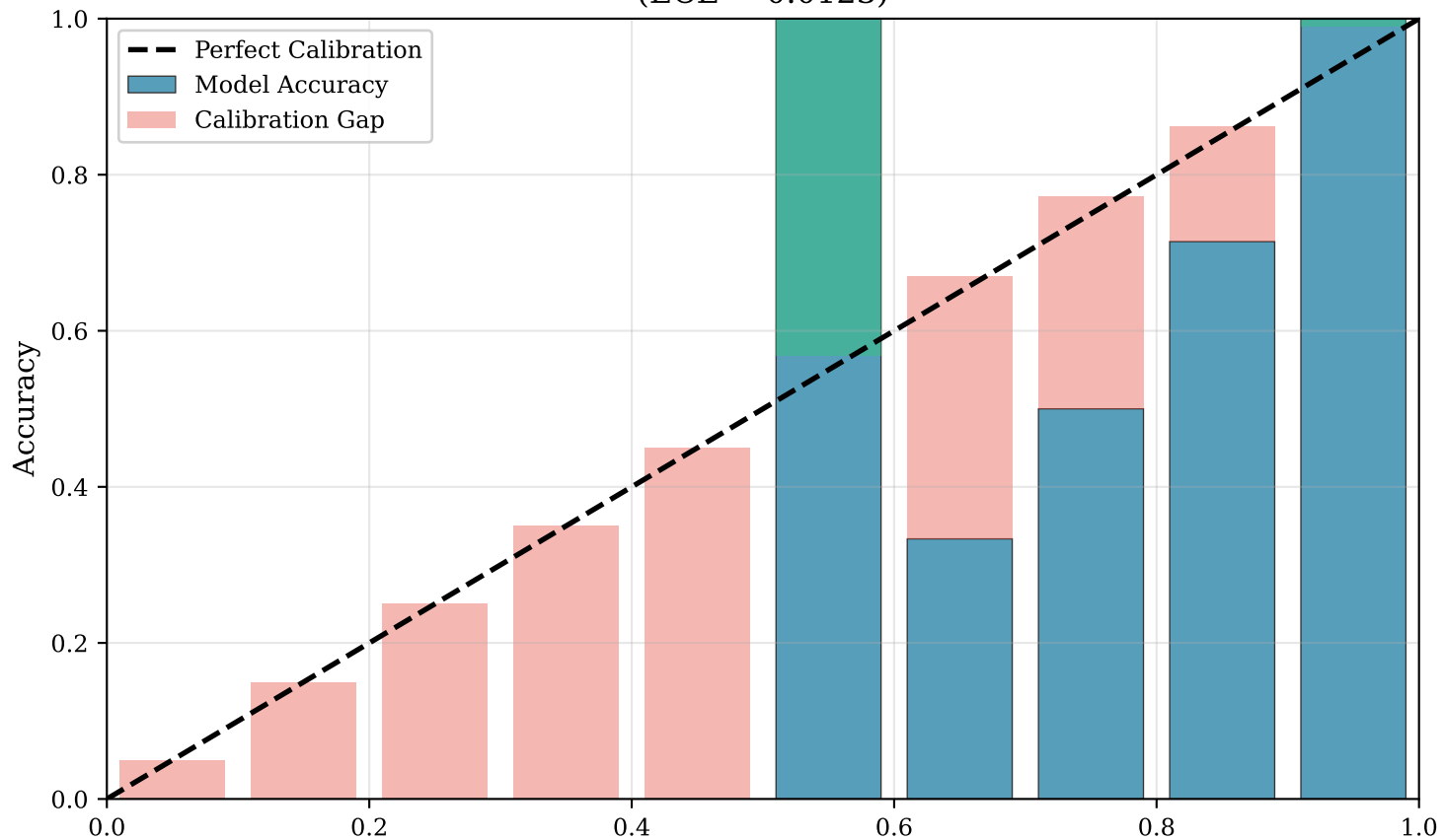
Reliability Diagram (ECE = 0.0123)
