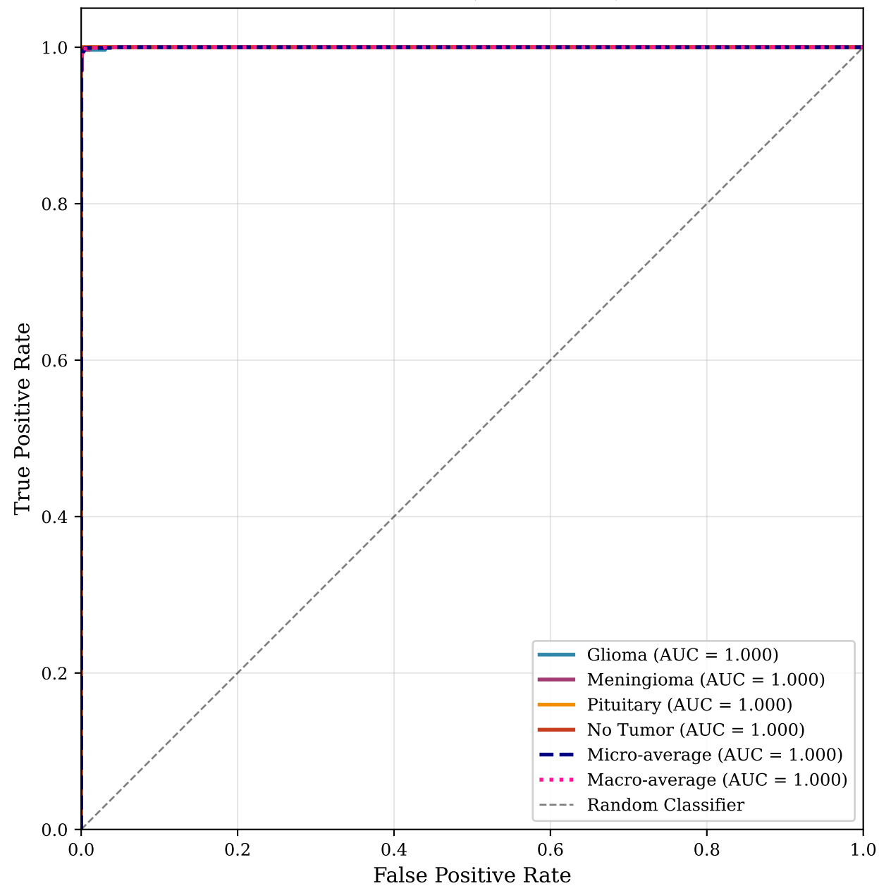
ROC Curves (One-vs-Rest)
