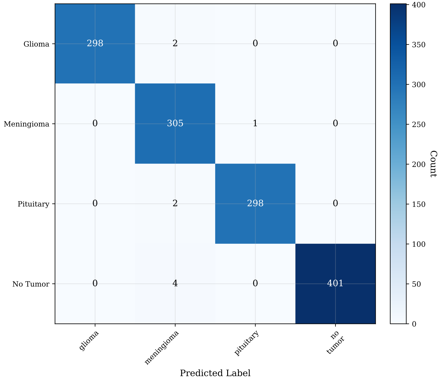
Confusion Matrix
