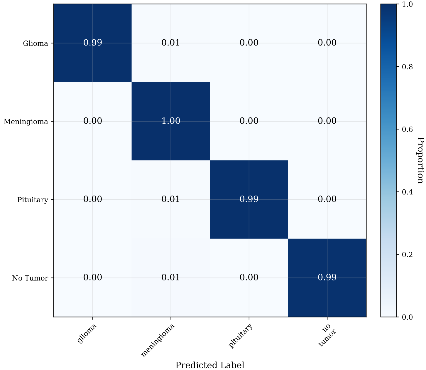
Confusion Matrix
