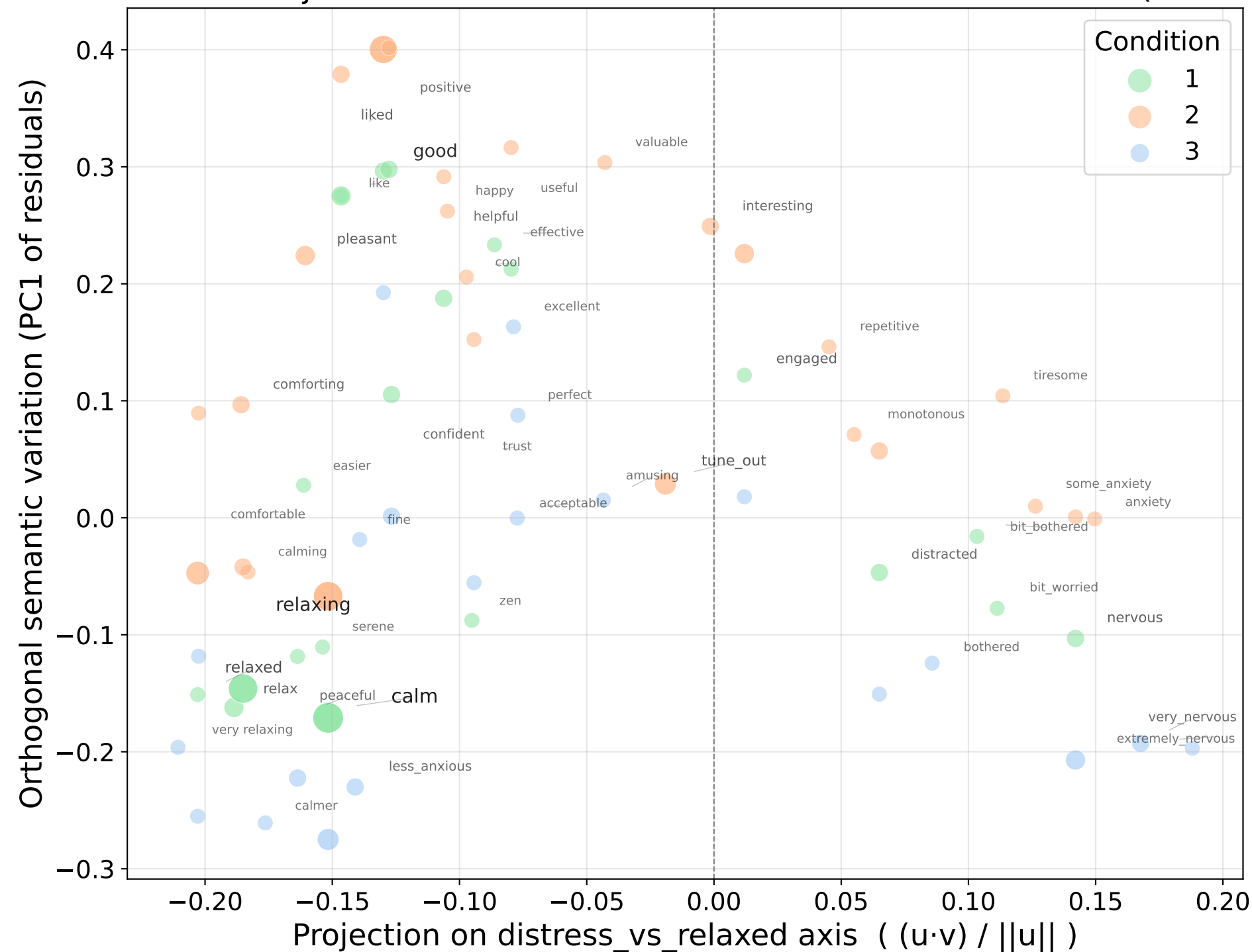
Semantic Projection of Emotional Words on Distress-Relaxed Axis (Gemini)
