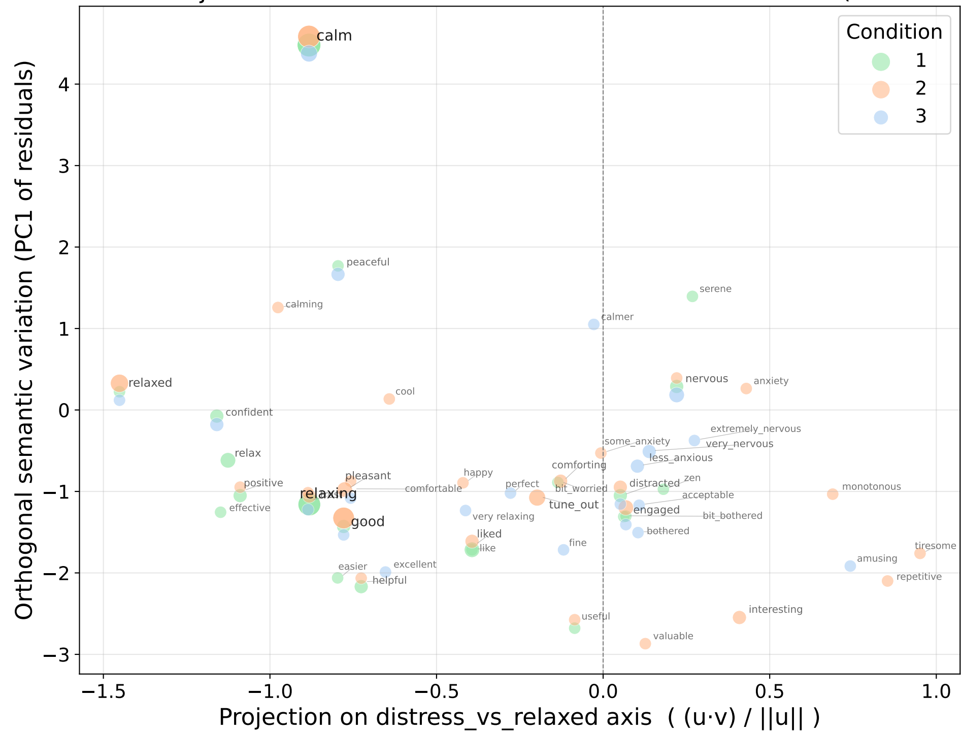
Semantic Projection of Emotional Words on Distress-Relaxed Axis (GloVe 300
