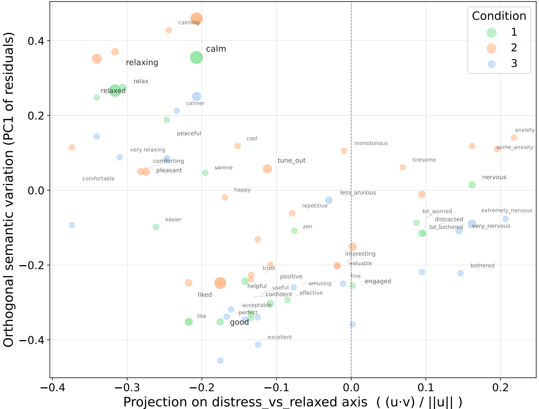
Semantic Projection of Emotional Words on Distress-Relaxed Axis (Jina v5 text-s
