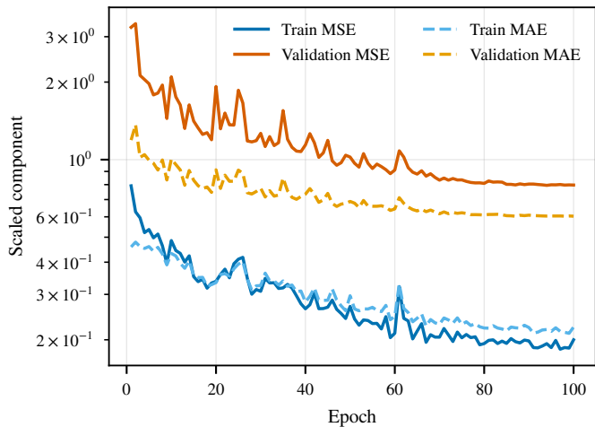
Data-loss components
