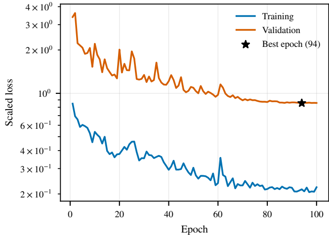
Residual-network objective
