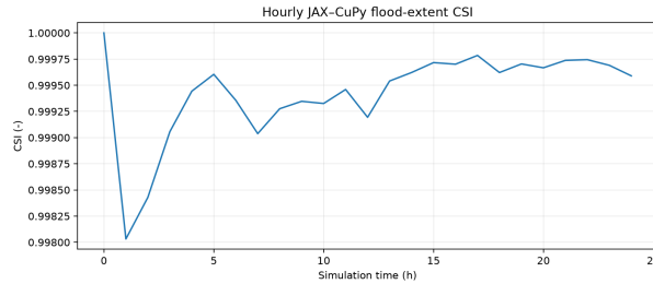
(b) Hourly flood-extent CSI.
