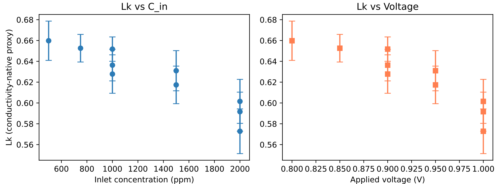
Fig. 3 — Lk Profile by Operating Condition (error bars = std over repeated cycles)
