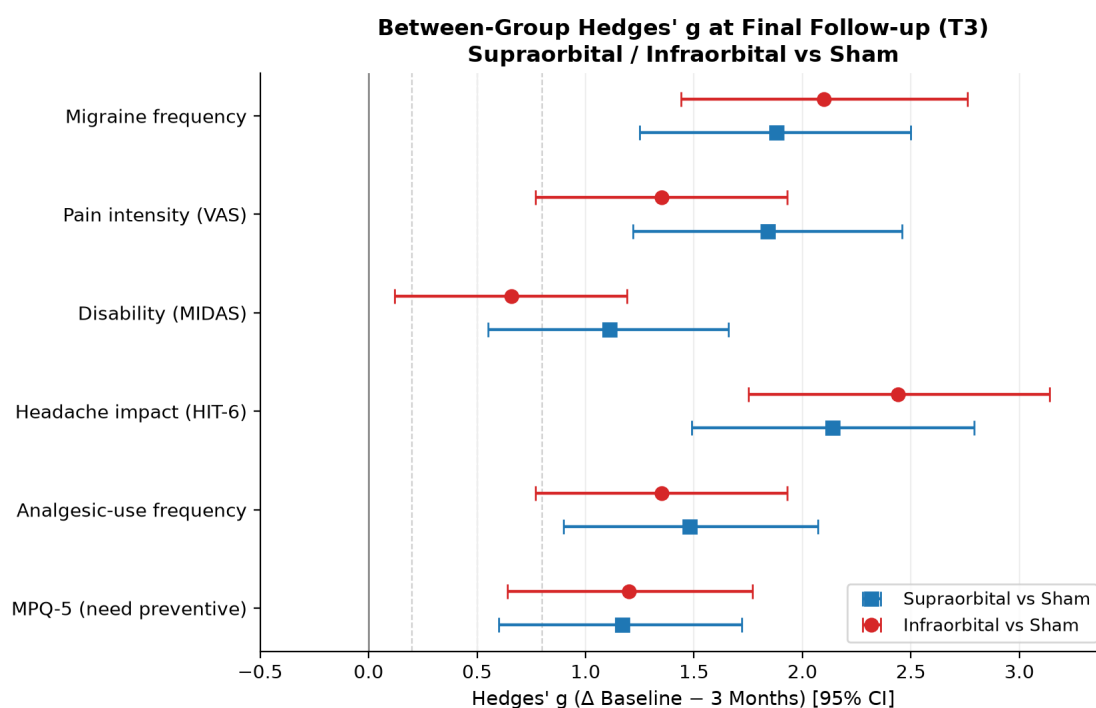
Figure 2. Between-group Hedges' g at final follow-up (T3): Supraorbital vs. Sham and Infraorbital vs. Sham, based on \Delta = \text{Baseline} - 3 \text{ Months} (Table 10 data). Squares/circles denote point estimates; horizontal lines denote 95% confidence intervals.
