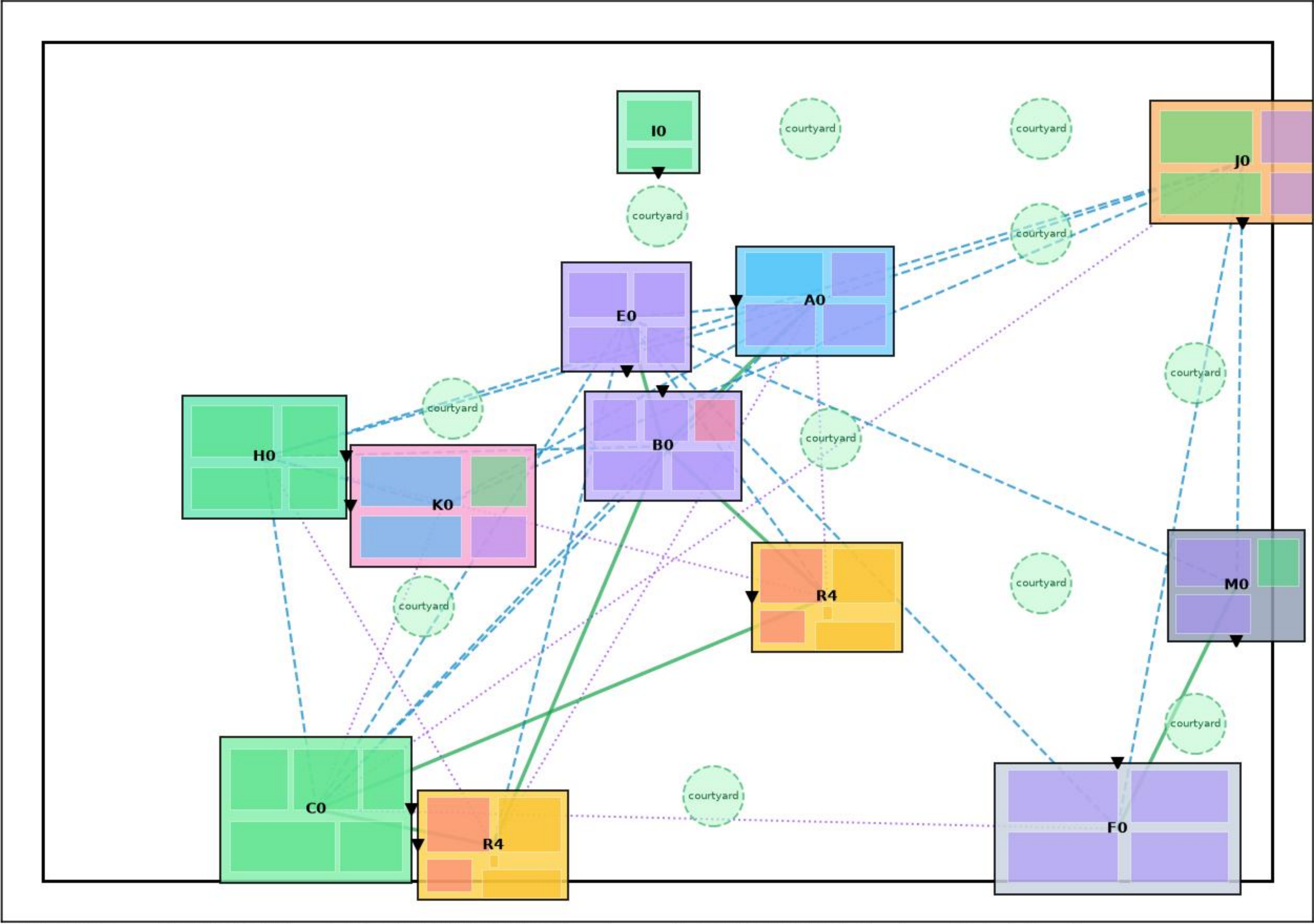
Schematic plan — A_BALANCED (rep 2, seed 42) R4x2 res=8 day=32 · GFA 1377 m 2 · landscape 53%
