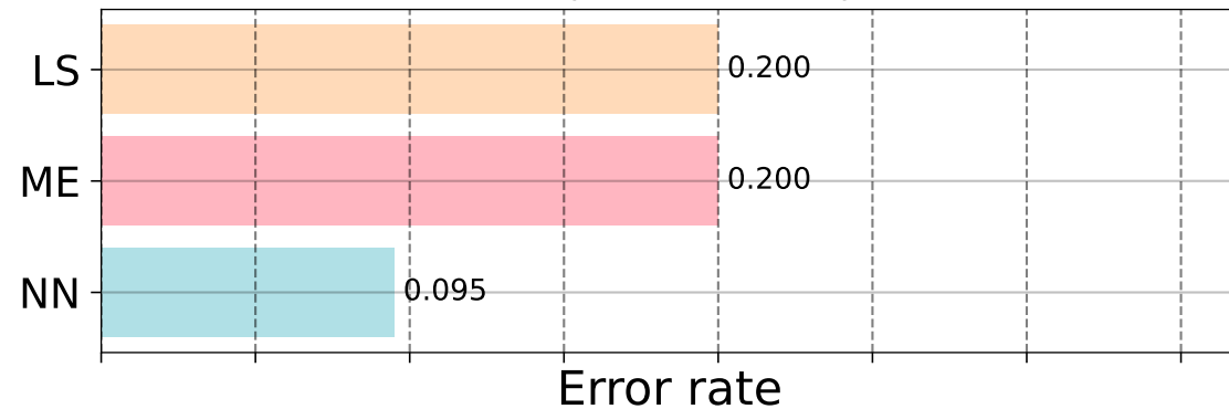
d = 2, features 2, 3
