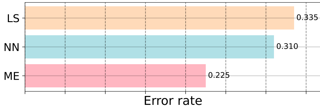
d = 1, features 2
