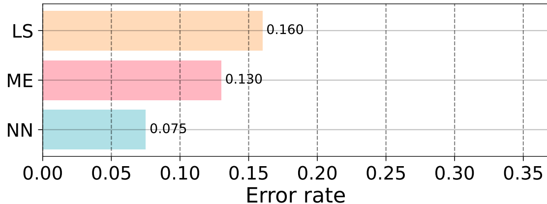
d = 3, features 2, 3, 4
