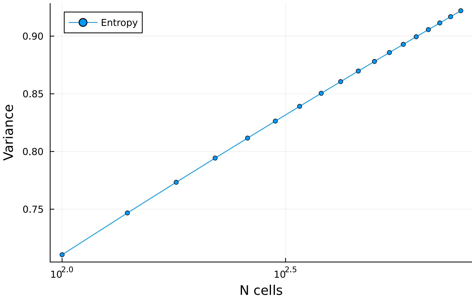
Variance vs N cells for gap \sim 0 - semilogx
