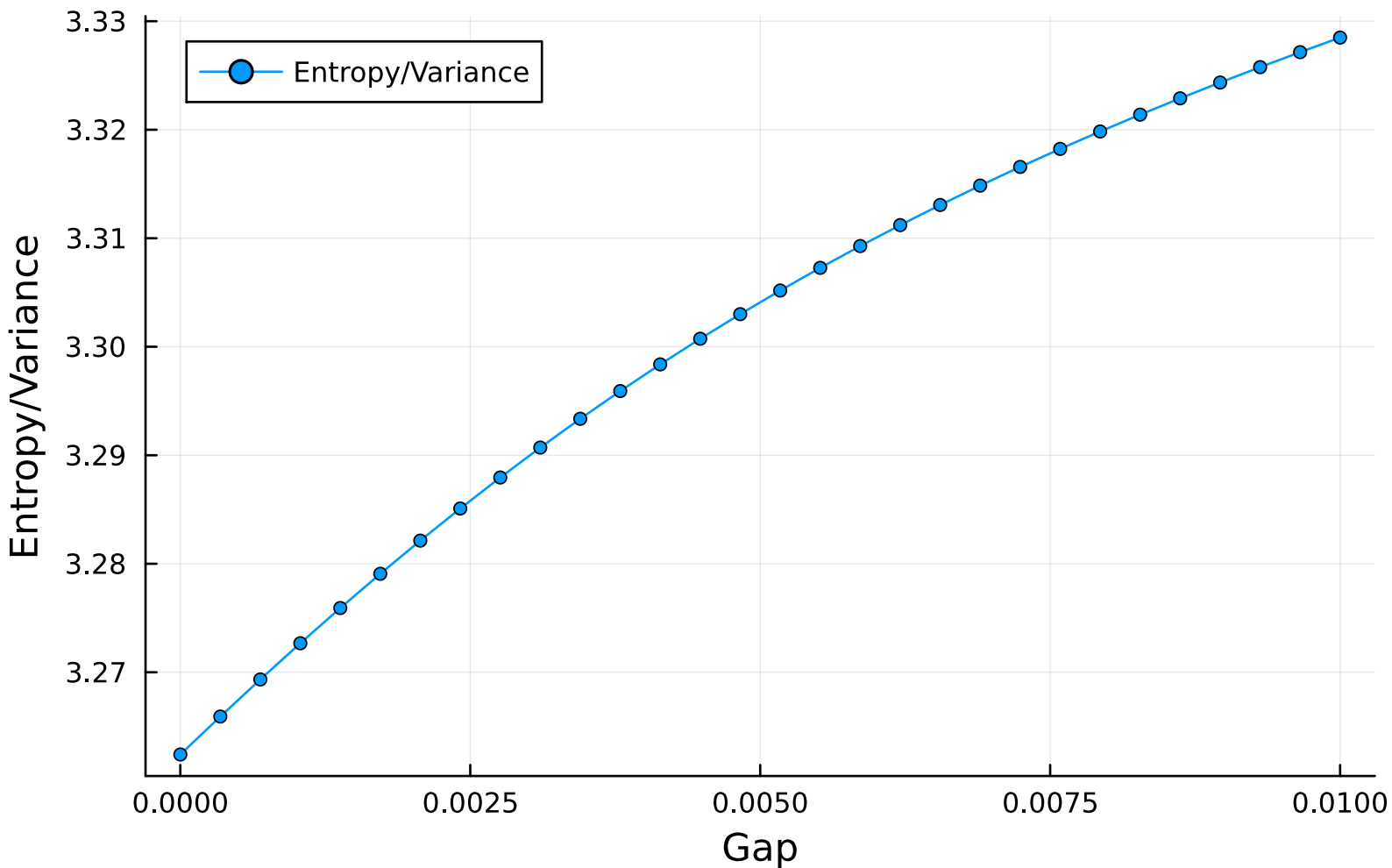
Entropy/Variance vs Gap for SSH model
