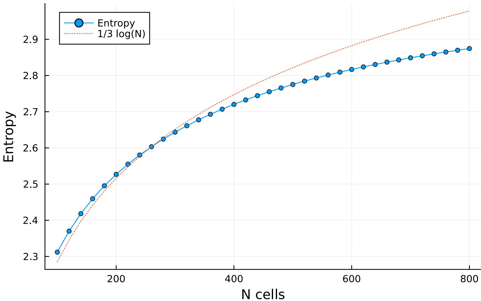
Entropy vs N cells for gap \sim 0
