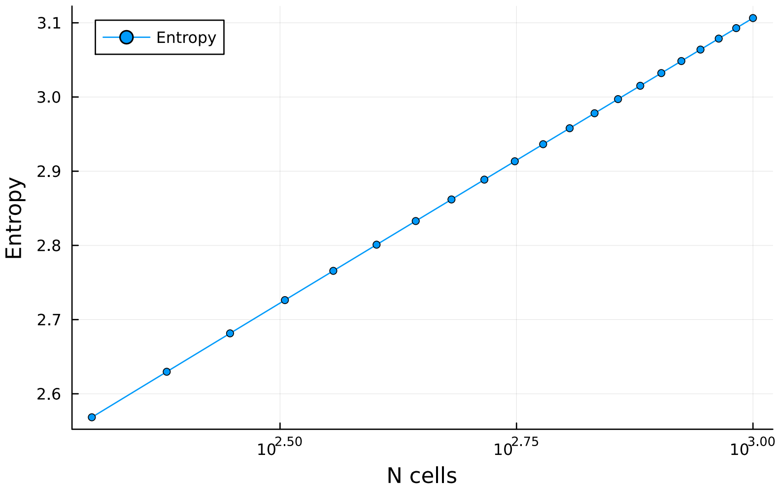
Entropy vs N cells for gap \sim 0 - semilogx
