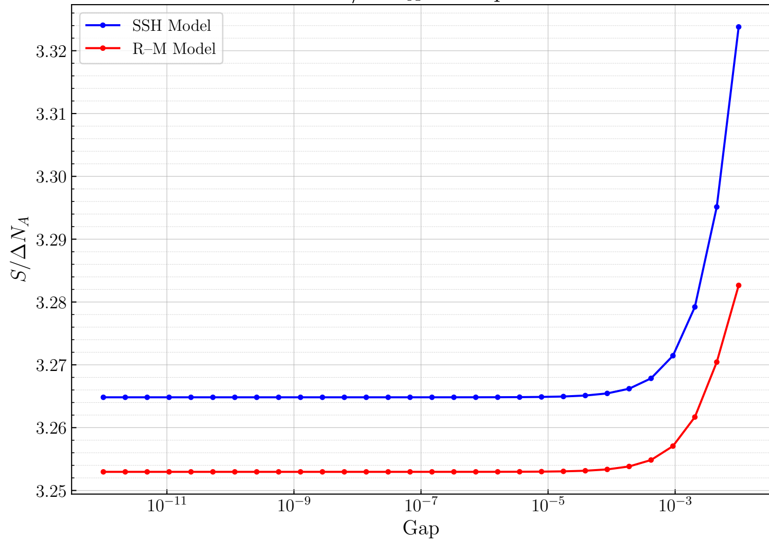
S/\Delta N_A vs Gap
