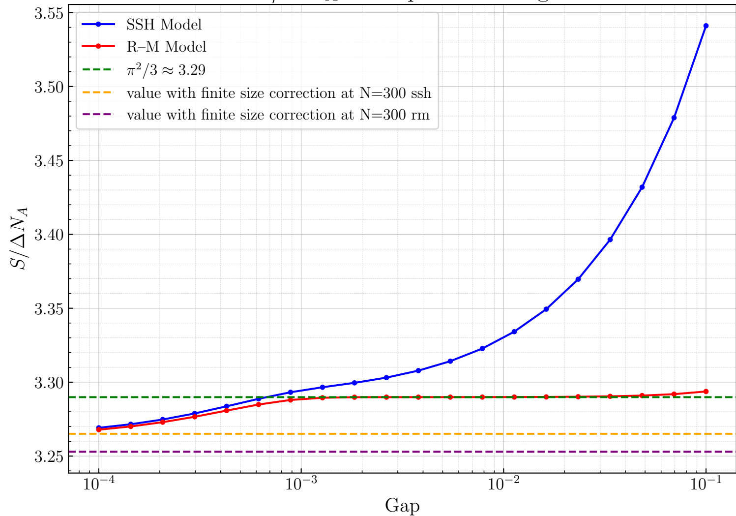
S/\Delta N_A vs Gap - half filling
