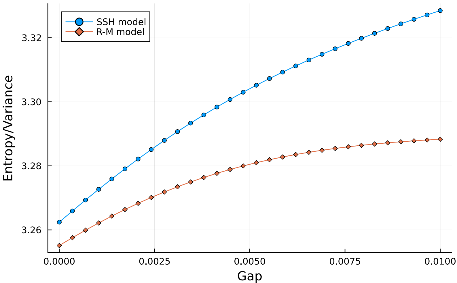
Entropy/Variance vs Gap for SSH and R-M models
