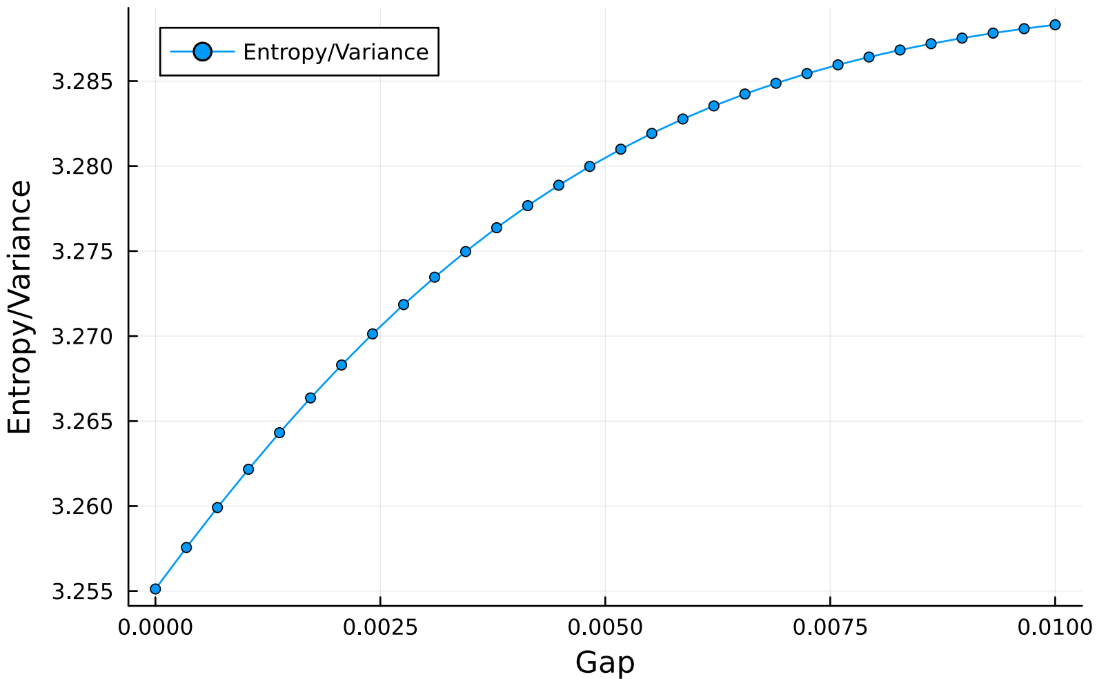
Entropy/Variance vs Gap for R-M model
