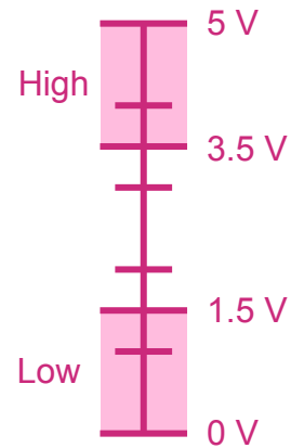
Acceptable CMOS input signal levels
