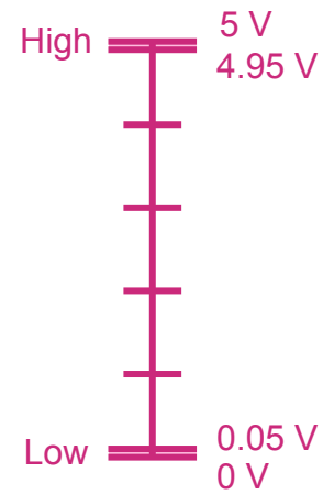
Acceptable CMOS output signal levels
