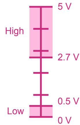
Acceptable TTL output signal levels
