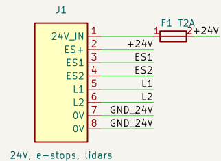
24V, e-stops, lidars
