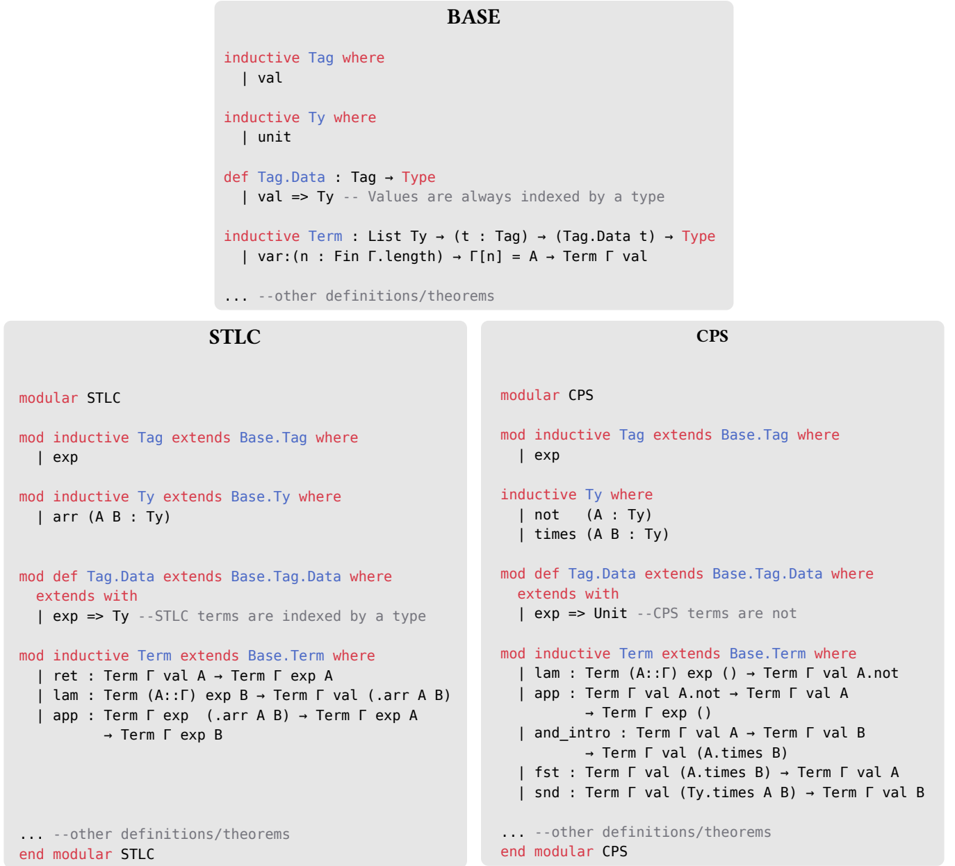
Figure 1: Definitions of Base, STLC and CPS, Term is indexed by a data associated to, this data gets extended accordingly for each extension.
