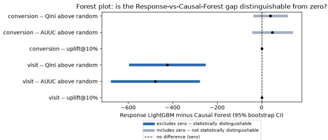
Figure 4 -- Forest plot: is the Response-vs-Causal-Forest gap distinguishable from zero?
