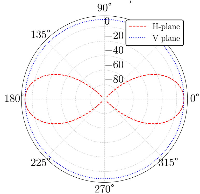
Cosine Pattern V/H Plane
