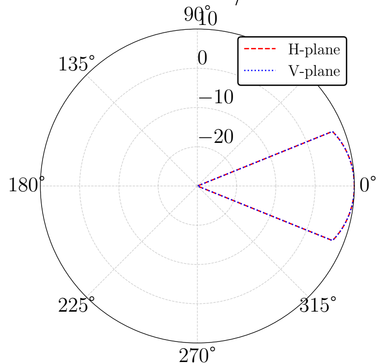
Ideal Pattern V/H Plane
