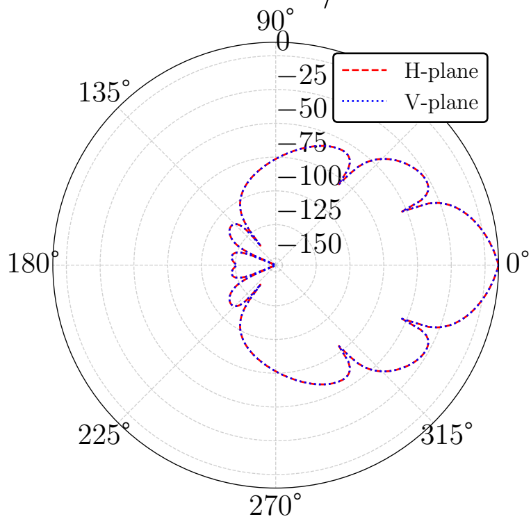
Sinc Pattern V/H Plane
